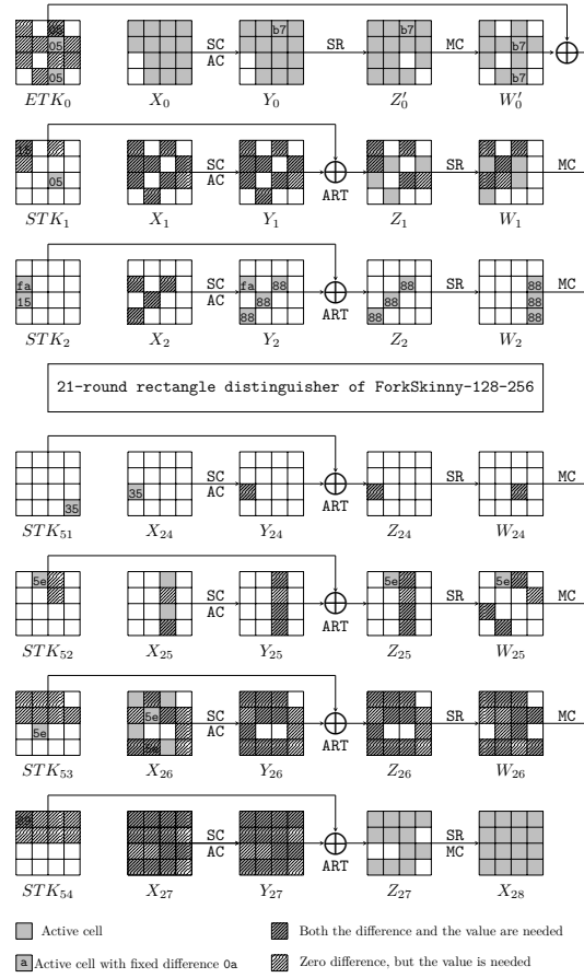
Figure 12: The 28-round attack against ForkSkinny-128-256 (256-bit key).
