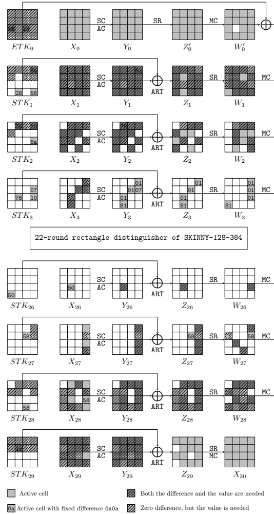
Figure 9: The 30-round attack against SKINNY-128-384.
