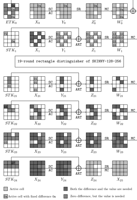
Figure 10: The 25-round attack against SKINNY-128-256.
